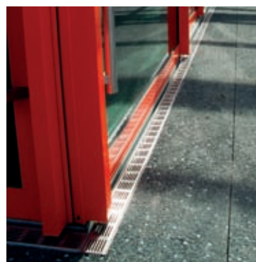
ABOVE: ACO Drain and deep pan access covers
